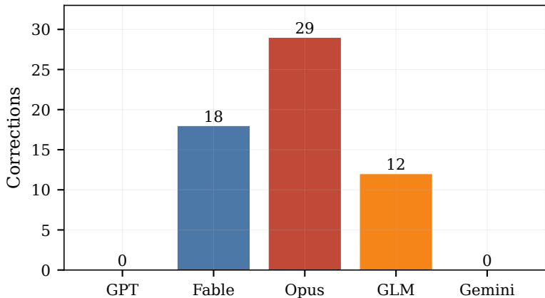
Self-Correction Frequency
