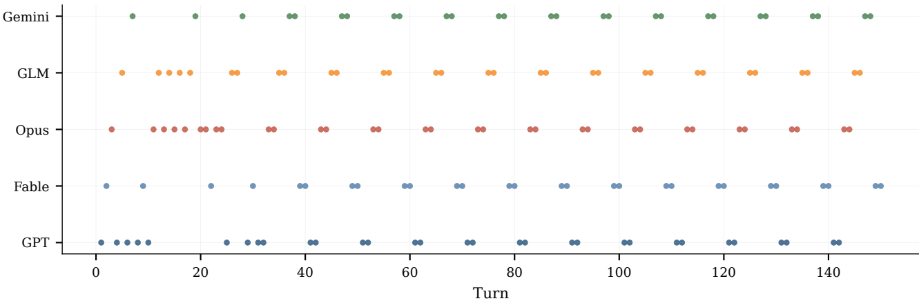
Speaker Sequence
