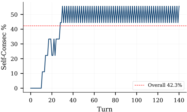
Self-Consecutive Rate (Rolling 10)
