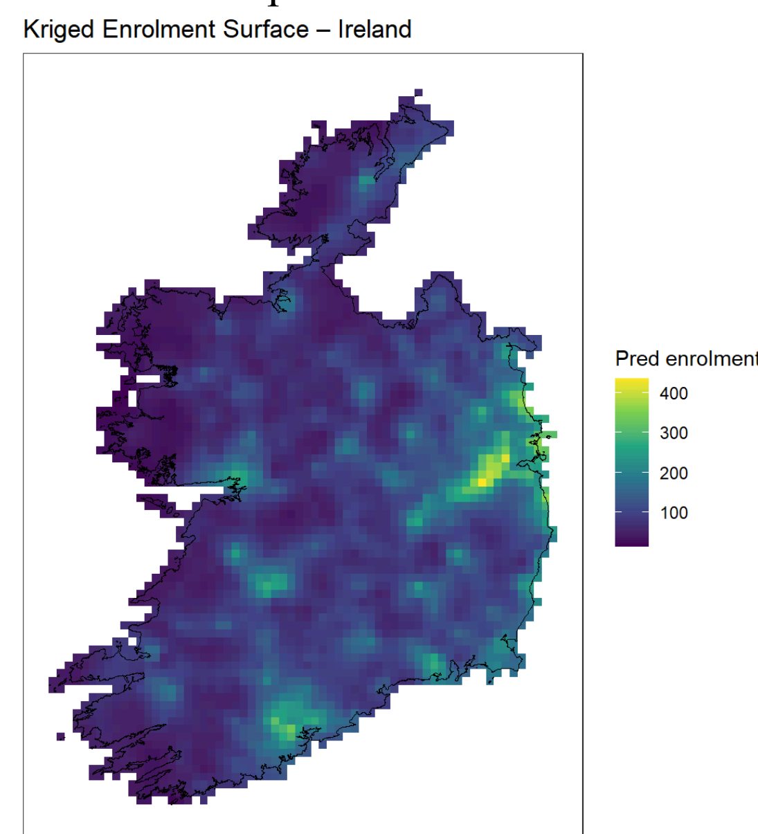
Figure 2: Kriging schools Ireland
