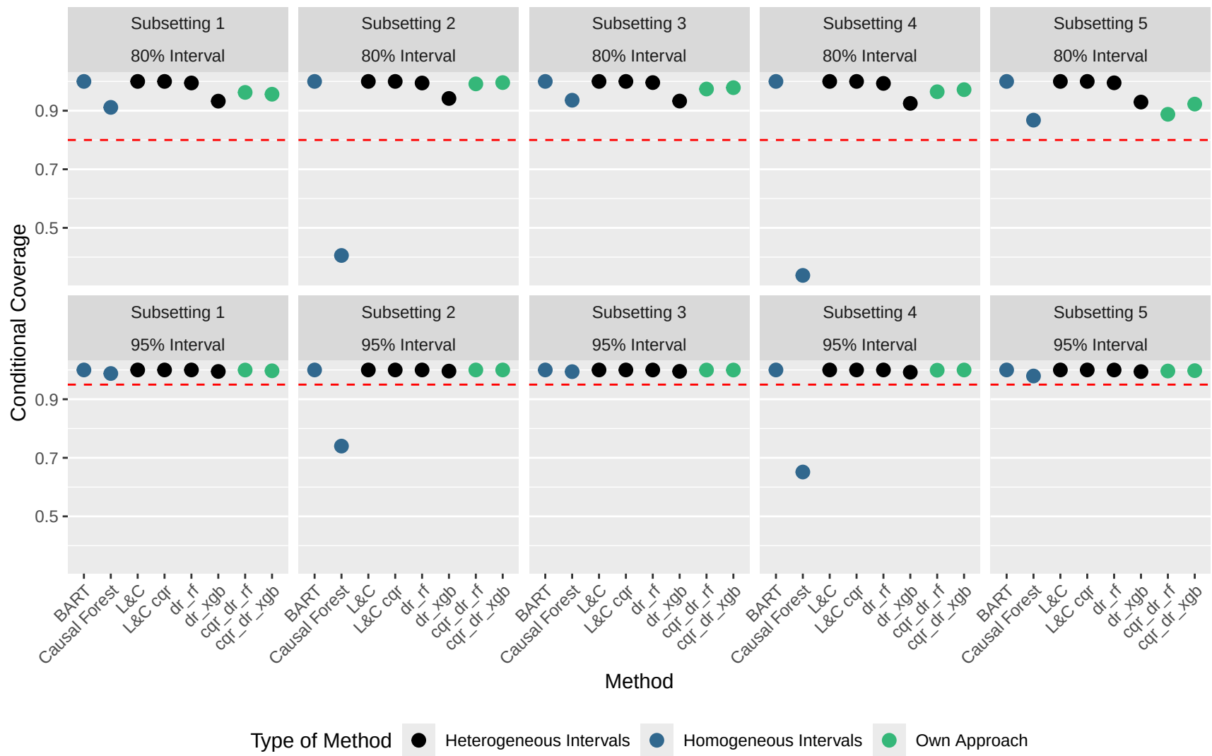
Conditional Coverage by Method
