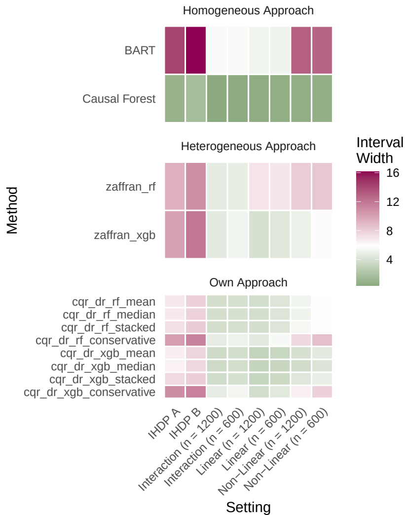
80% Interval (MAR)
