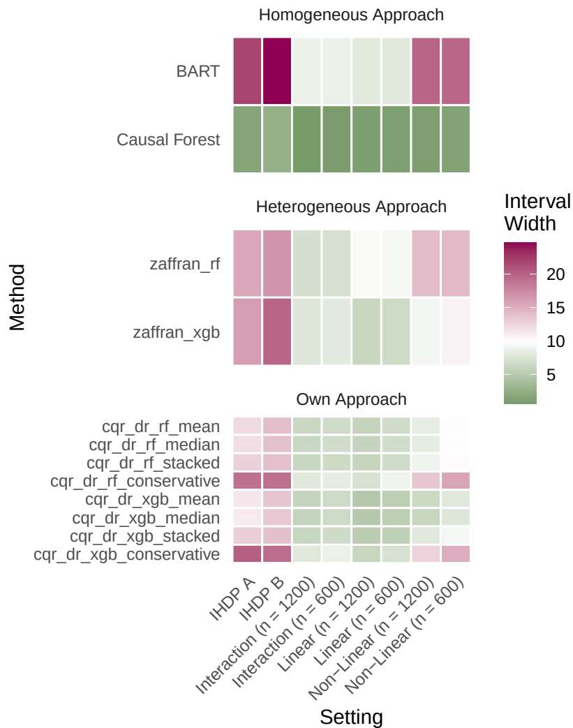
95% Interval (MAR)
