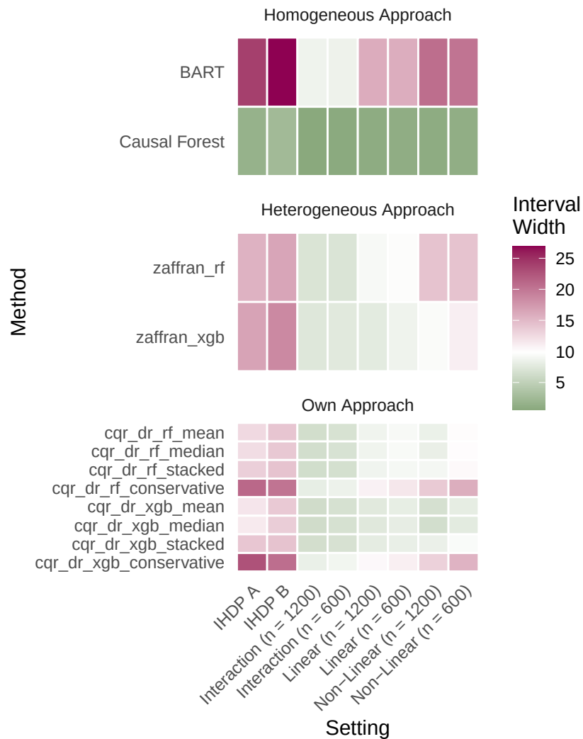
95% Interval (MCAR)
