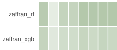
Own Approach
