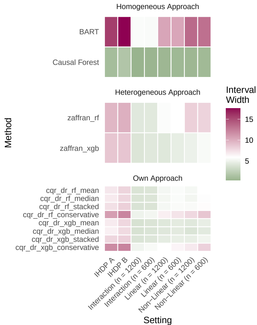
80% Interval (MCAR)
