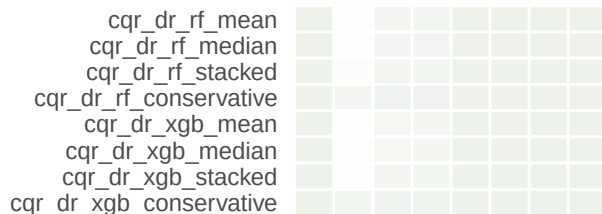
Own Approach
