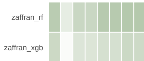
Own Approach
