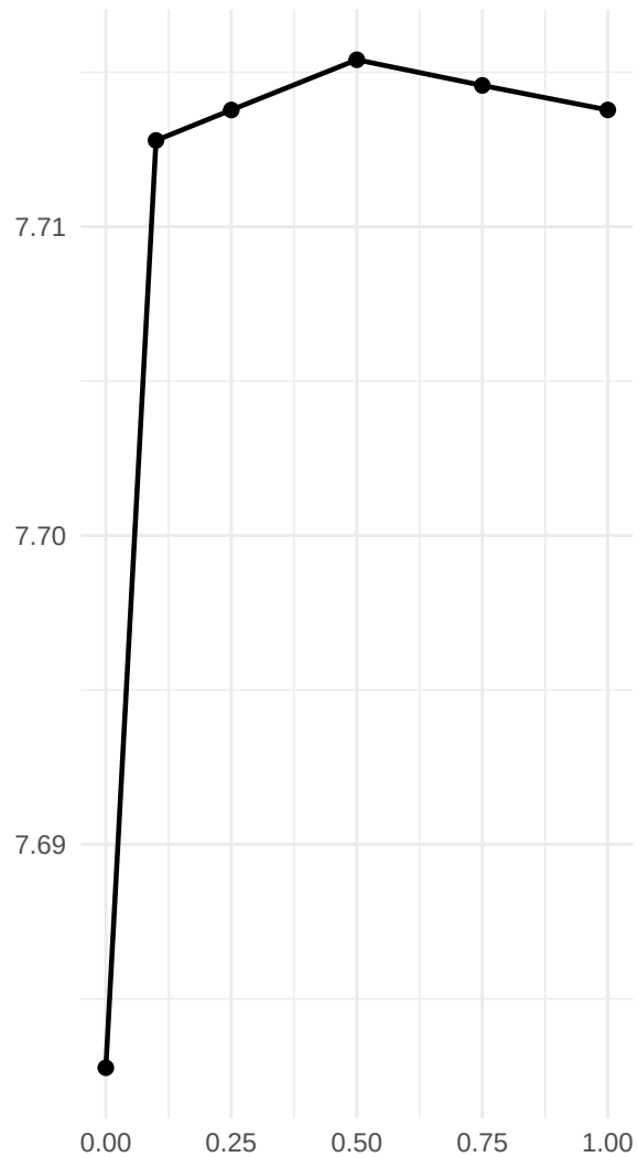
Policy value
