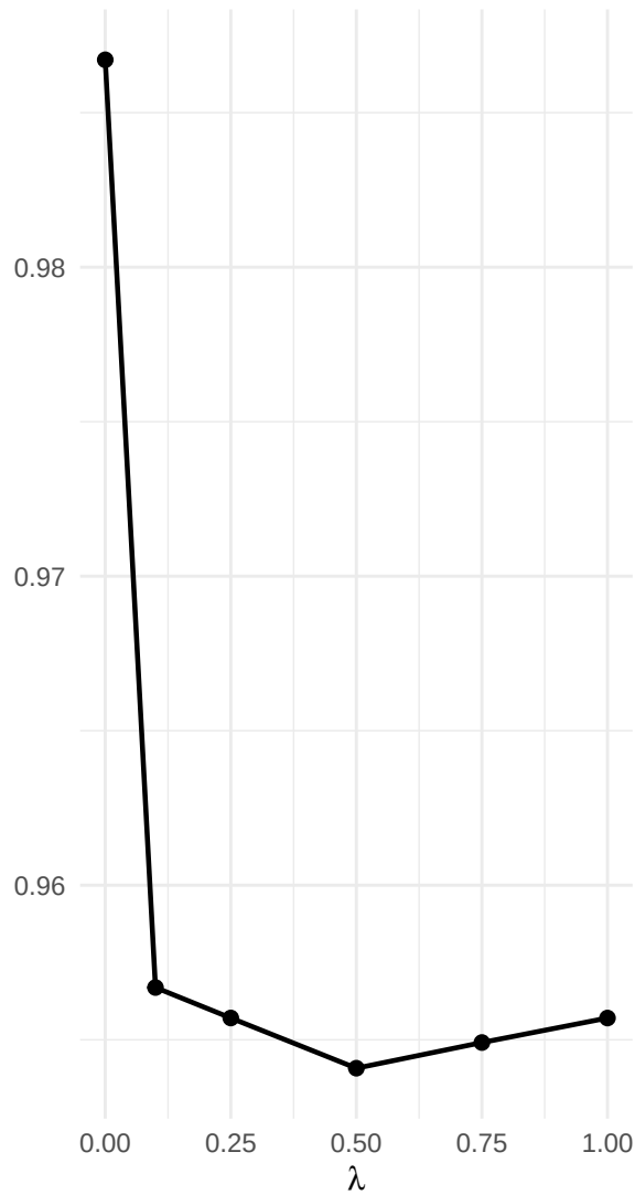
Mean regret
