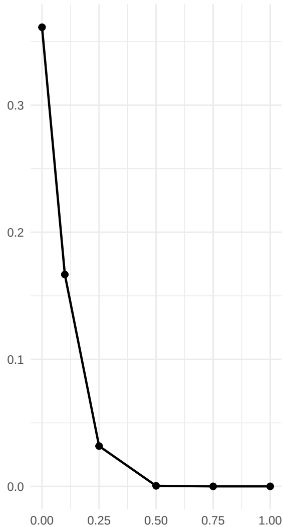
Harm rate
