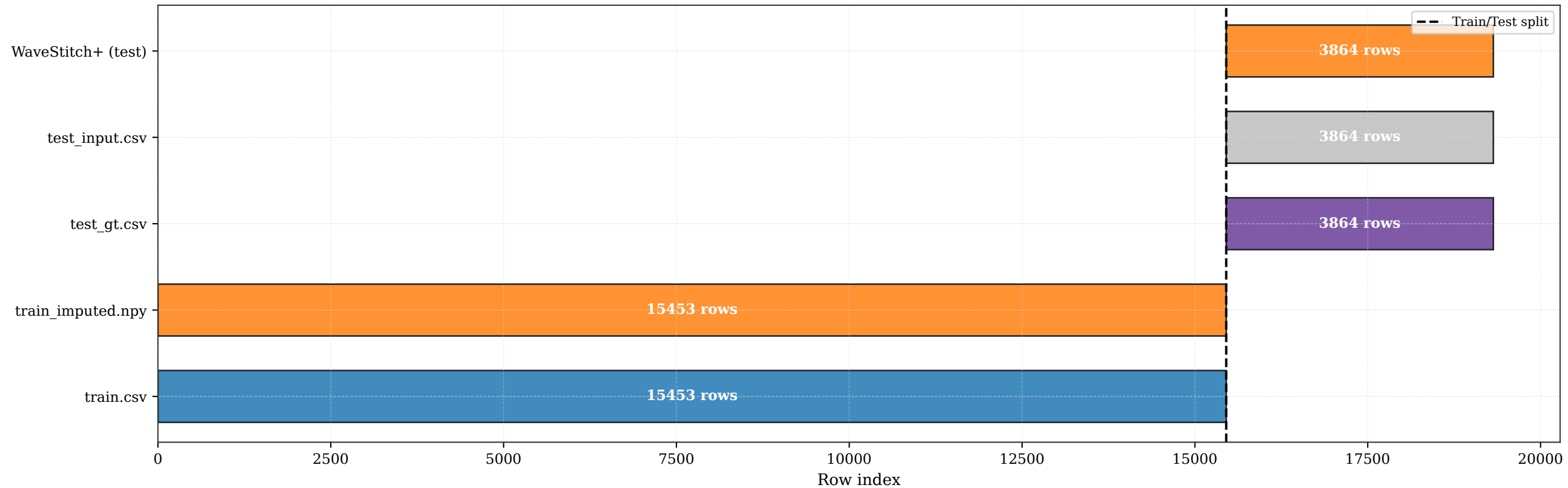
golang — Data layout overview
