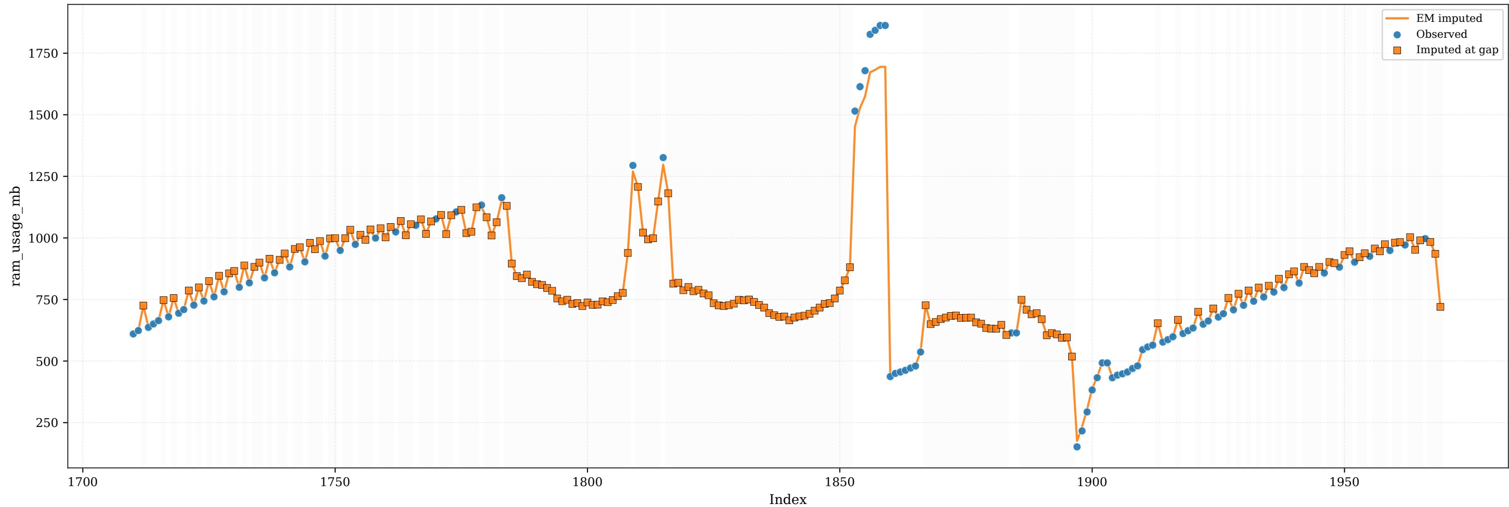
ram_usage_mb — Overlay comparison (idx 1710-1970)
