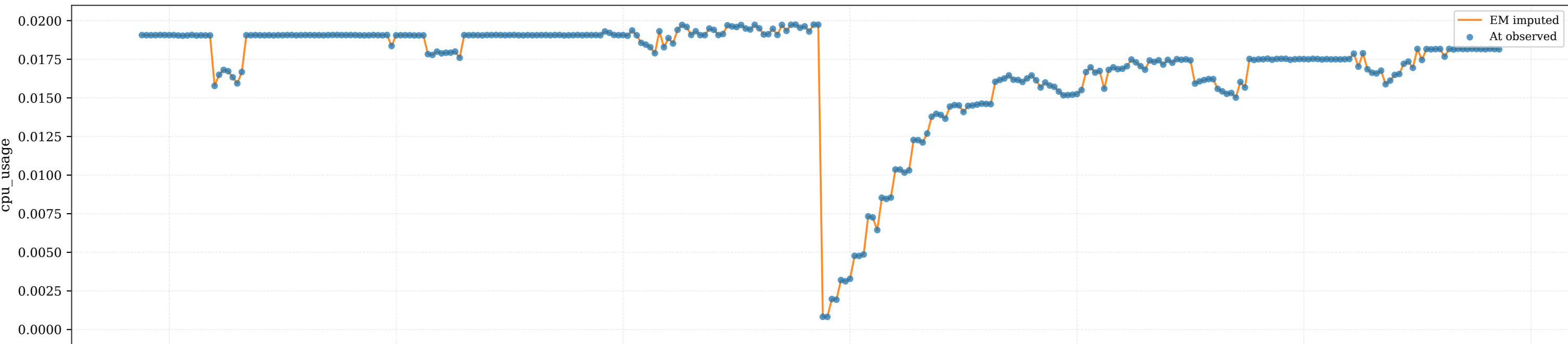
EM-imputed train data
