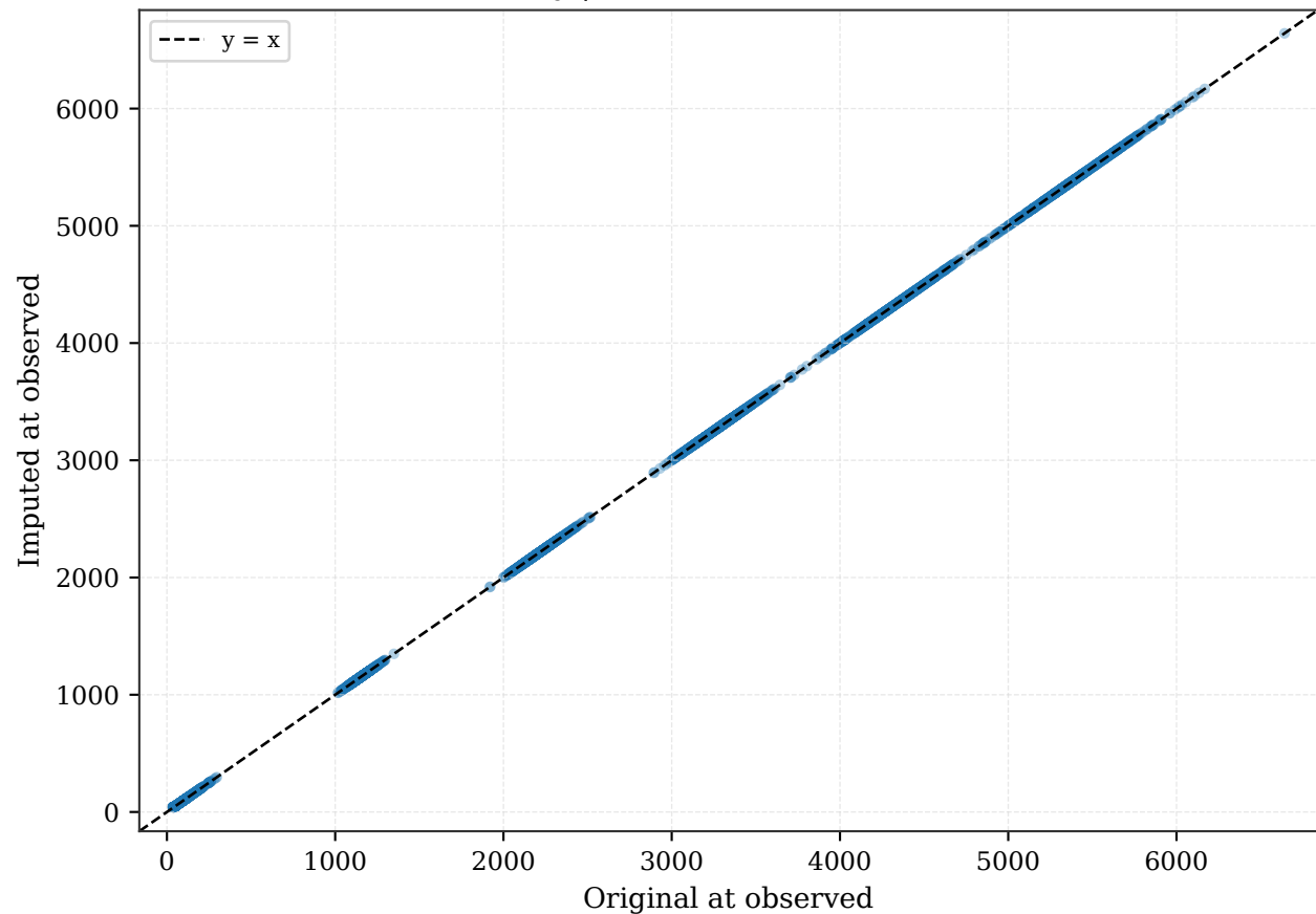
Consistency | Corr=1.0000, MAE=0.025325
