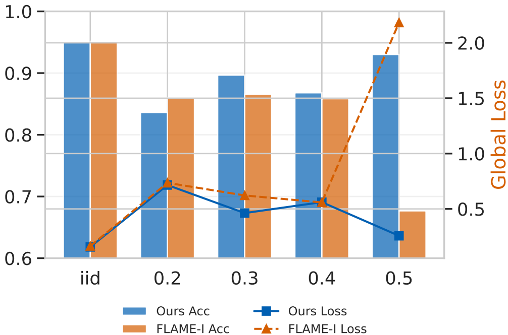
Global Accuracy
