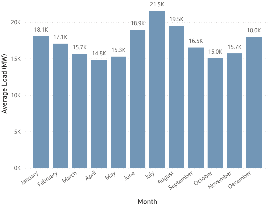
Average Electricity Load by Month (2024)
