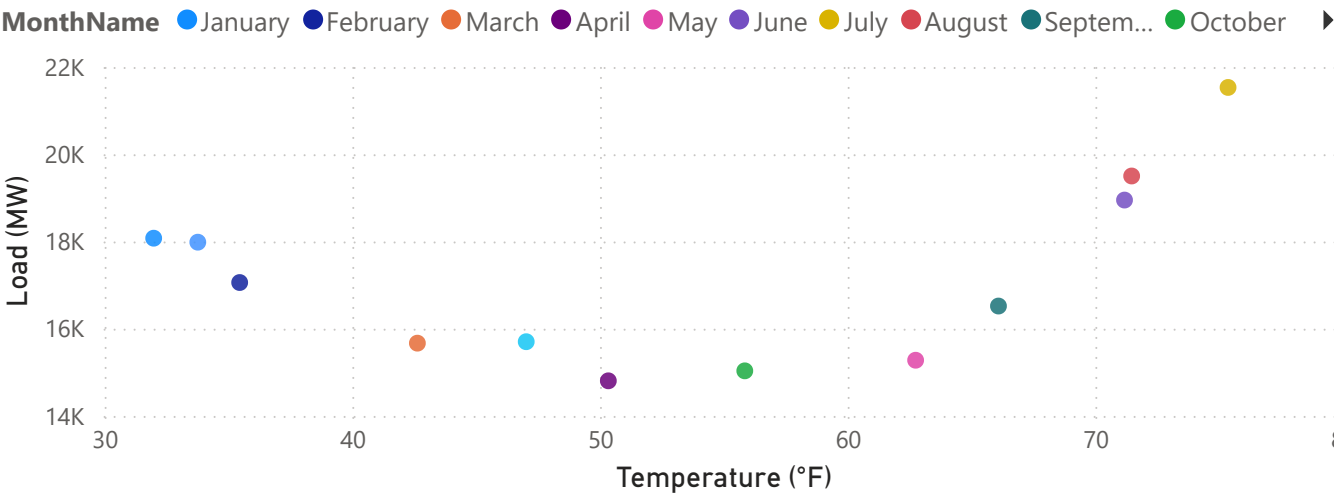
Temperature vs Electricity Load (2024)
