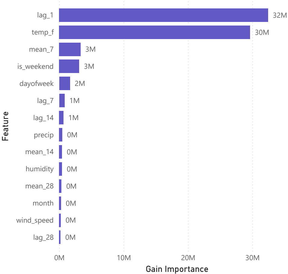
XGBoost Feature Importance (Gain Score)
