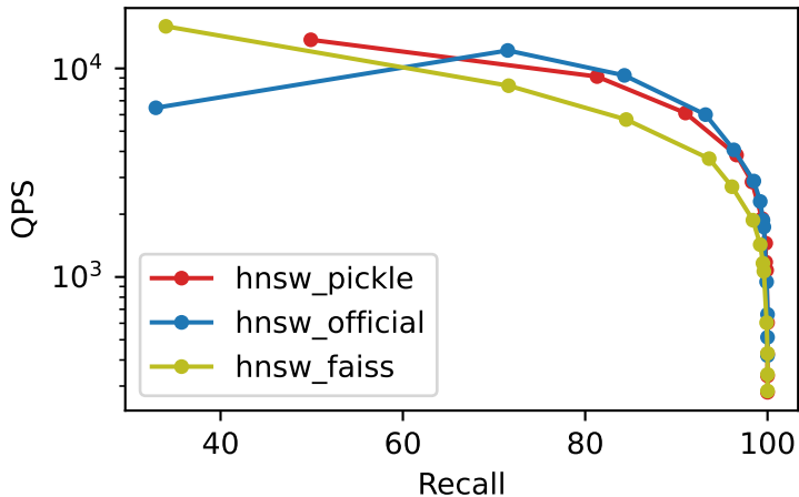
Recall vs QPS bigann_1M_M32_ef100_k1
