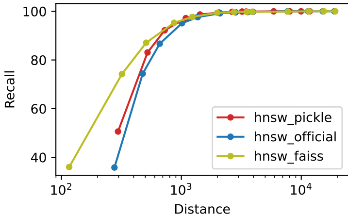
Recall vs Distance bigann_1M_M32_ef300_k1
