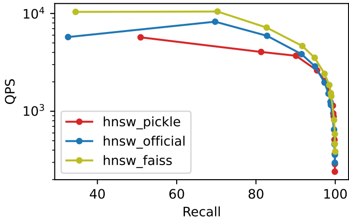
Recall vs QPS deep_1M_M32_ef100_k1
