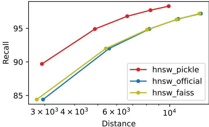
Recall vs Distance text2image_1M_M32_ef100_k100
