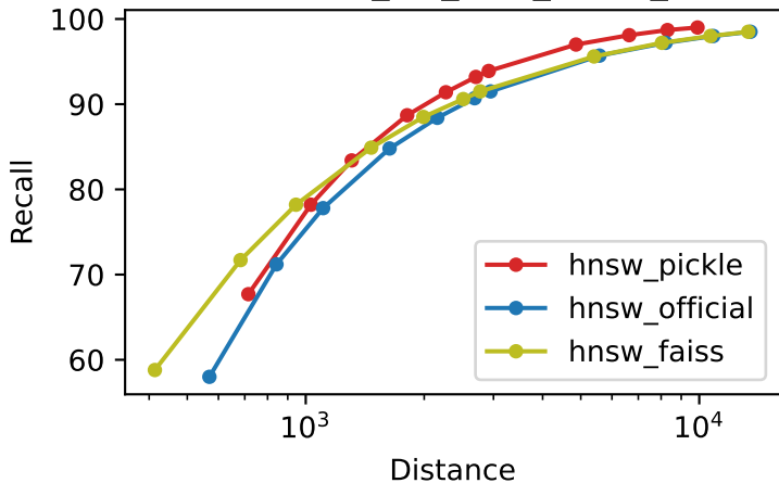
Recall vs Distance text2image_1M_M32_ef100_k10
