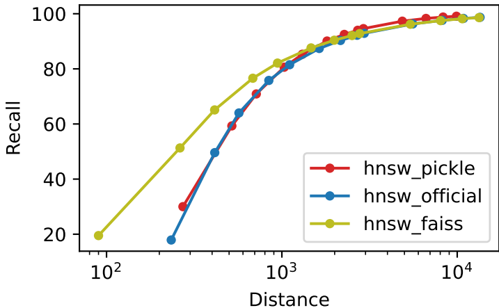
Recall vs Distance text2image_1M_M32_ef100_k1
