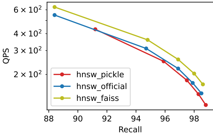
Recall vs QPS text2image_1M_M32_ef300_k100
