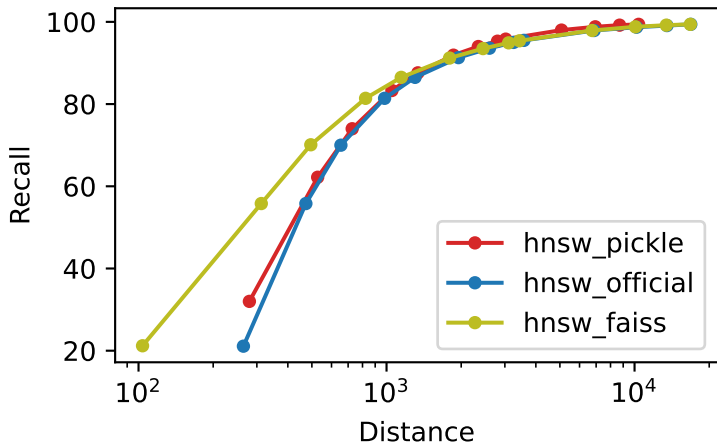
Recall vs Distance text2image_1M_M32_ef300_k1
