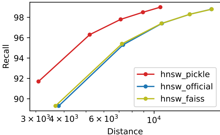
Recall vs Distance text2image_1M_M32_ef500_k100
