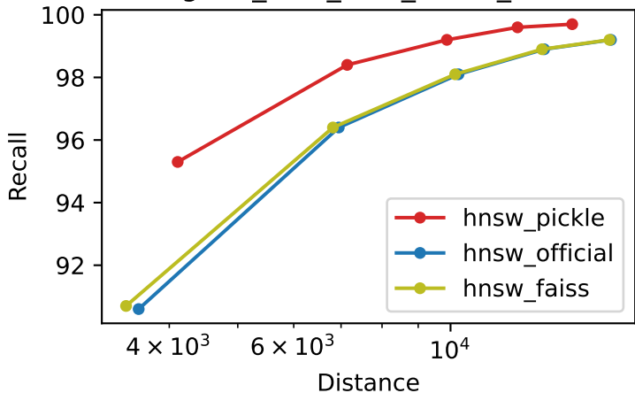
Recall vs Distance bigann_10M_M32_ef100_k100
