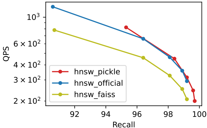
Recall vs QPS bigann_10M_M32_ef100_k100
