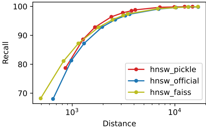
Recall vs Distance bigann_10M_M32_ef100_k10
