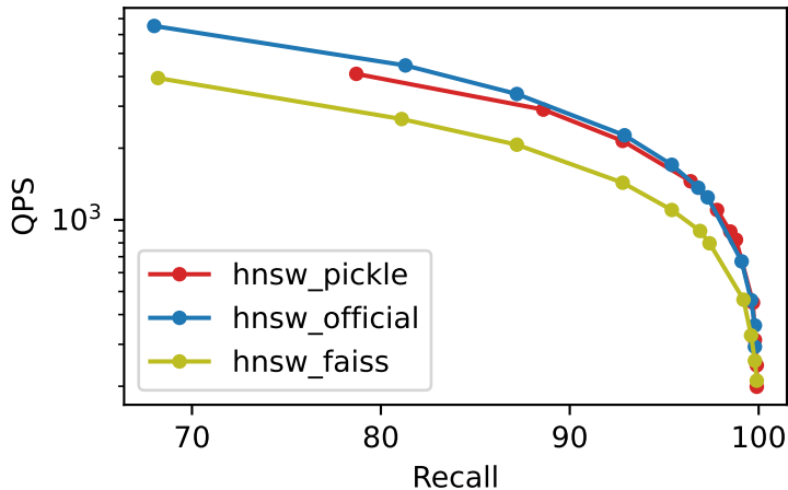
Recall vs QPS bigann_10M_M32_ef100_k10
