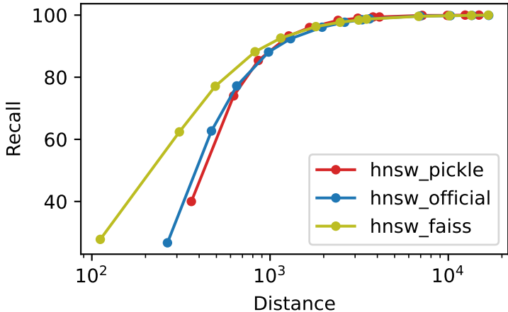
Recall vs Distance bigann_10M_M32_ef100_k1
