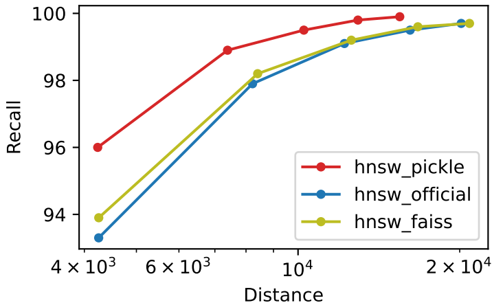
Recall vs Distance bigann_10M_M32_ef300_k100
