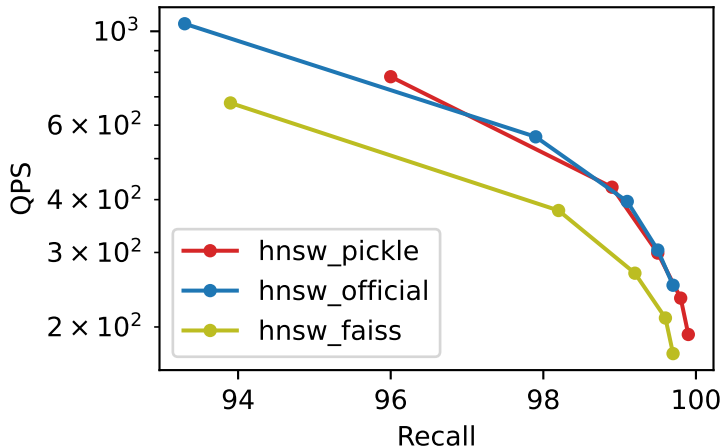
Recall vs QPS bigann_10M_M32_ef300_k100
