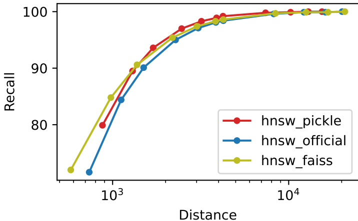
Recall vs Distance bigann_10M_M32_ef300_k10
