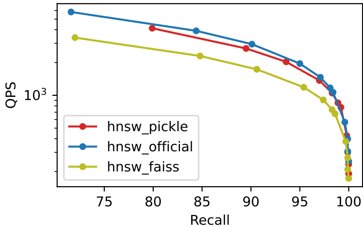
Recall vs QPS bigann_10M_M32_ef300_k10
