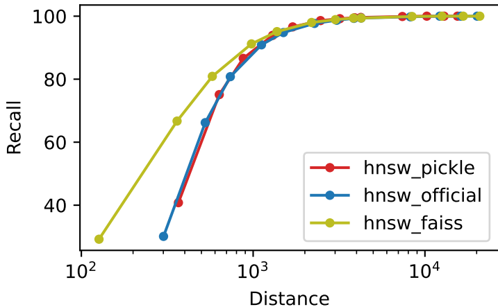
Recall vs Distance bigann_10M_M32_ef300_k1
