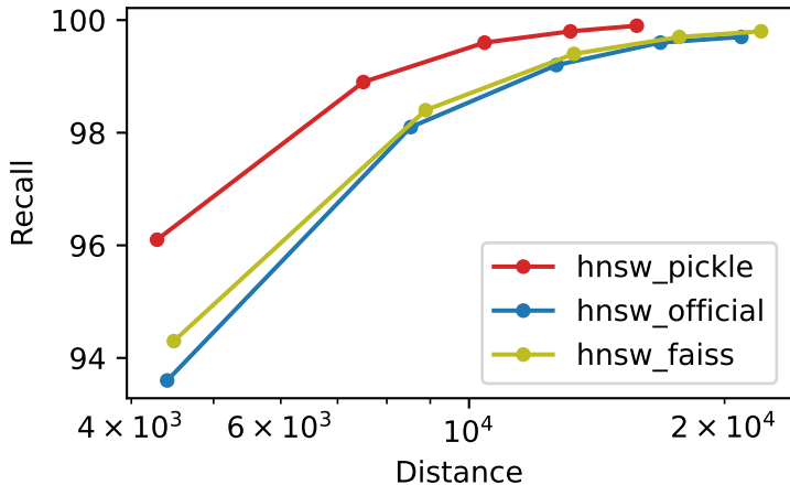
Recall vs Distance bigann_10M_M32_ef500_k100
