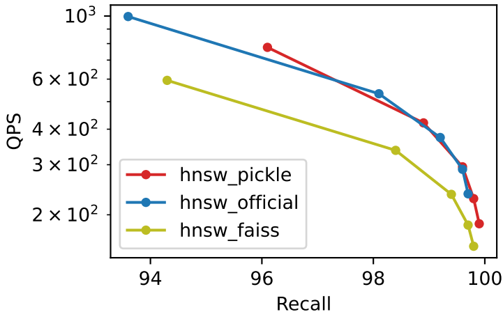
Recall vs QPS bigann_10M_M32_ef500_k100
