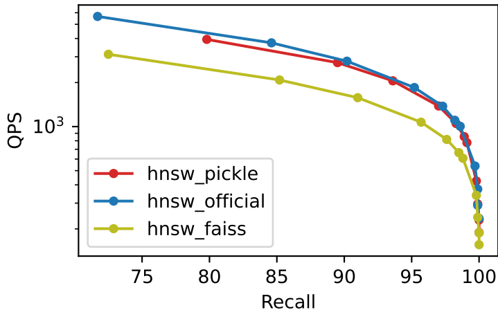
Recall vs QPS bigann_10M_M32_ef500_k10
