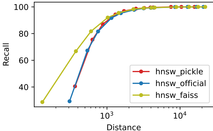
Recall vs Distance bigann_10M_M32_ef500_k1
