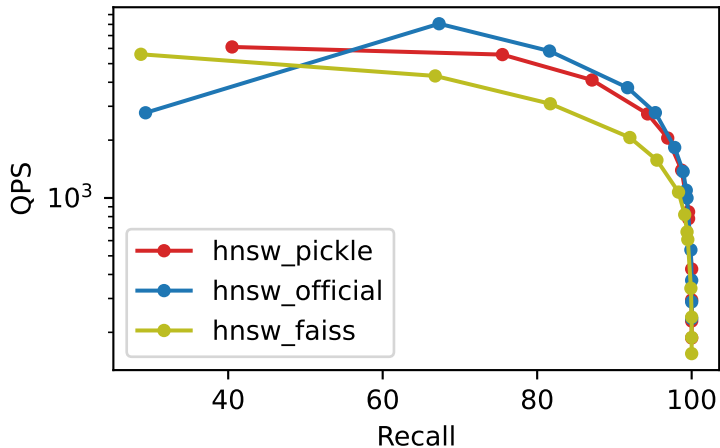
Recall vs QPS bigann_10M_M32_ef500_k1
