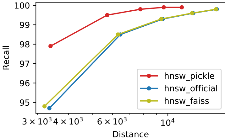
Recall vs Distance bigann_1M_M32_ef100_k100
