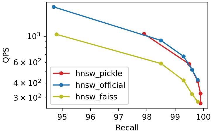
Recall vs QPS bigann_1M_M32_ef100_k100
