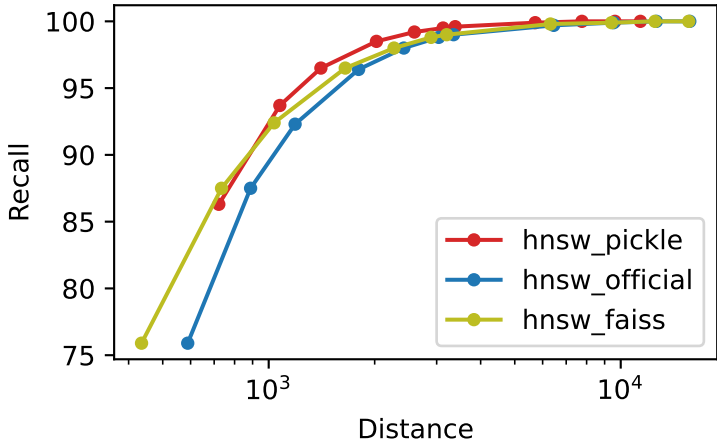
Recall vs Distance bigann_1M_M32_ef100_k10
