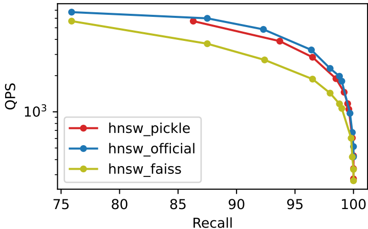
Recall vs QPS bigann_1M_M32_ef100_k10
