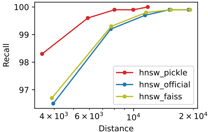
Recall vs Distance bigann_1M_M32_ef300_k100
