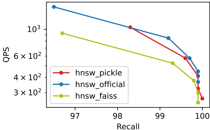
Recall vs QPS bigann_1M_M32_ef300_k100
