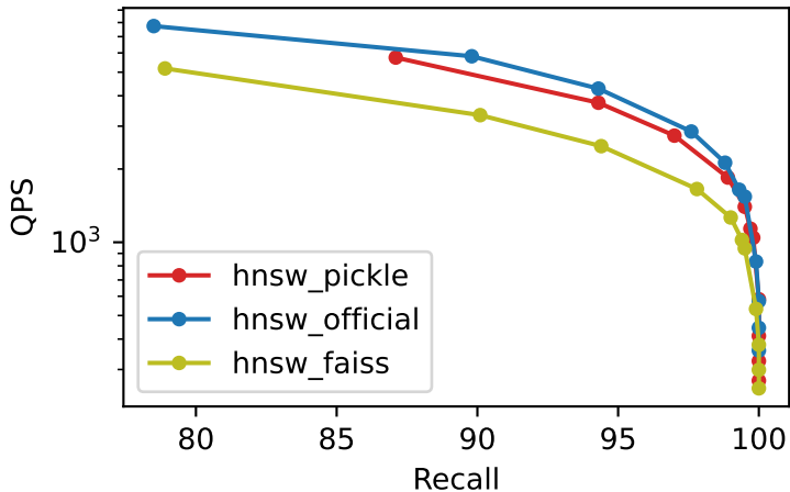
Recall vs QPS bigann_1M_M32_ef300_k10
