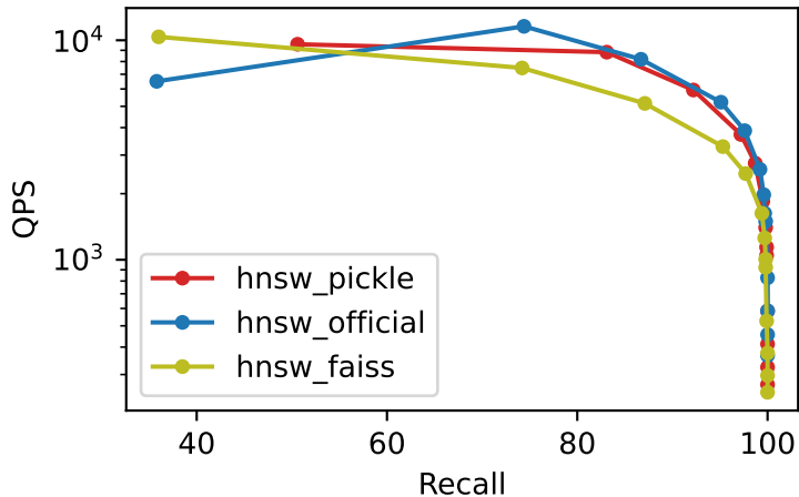
Recall vs QPS bigann_1M_M32_ef300_k1
