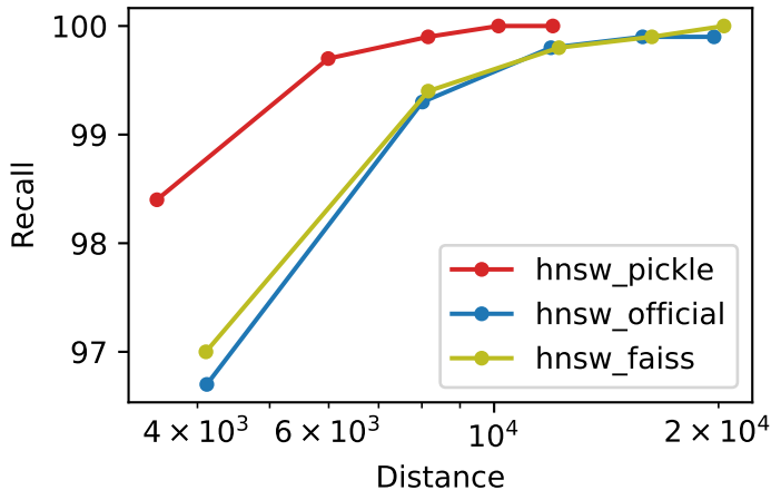
Recall vs Distance bigann_1M_M32_ef500_k100
