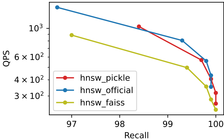
Recall vs QPS bigann_1M_M32_ef500_k100
