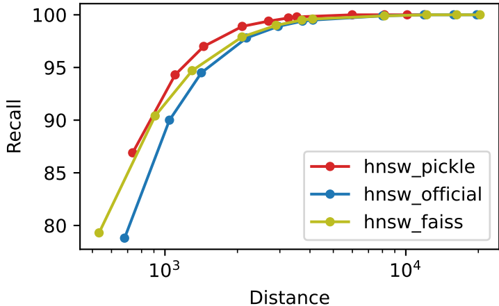
Recall vs Distance bigann_1M_M32_ef500_k10
