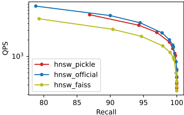
Recall vs QPS bigann_1M_M32_ef500_k10
