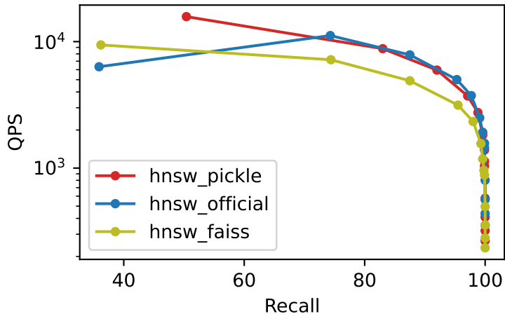
Recall vs QPS bigann_1M_M32_ef500_k1
